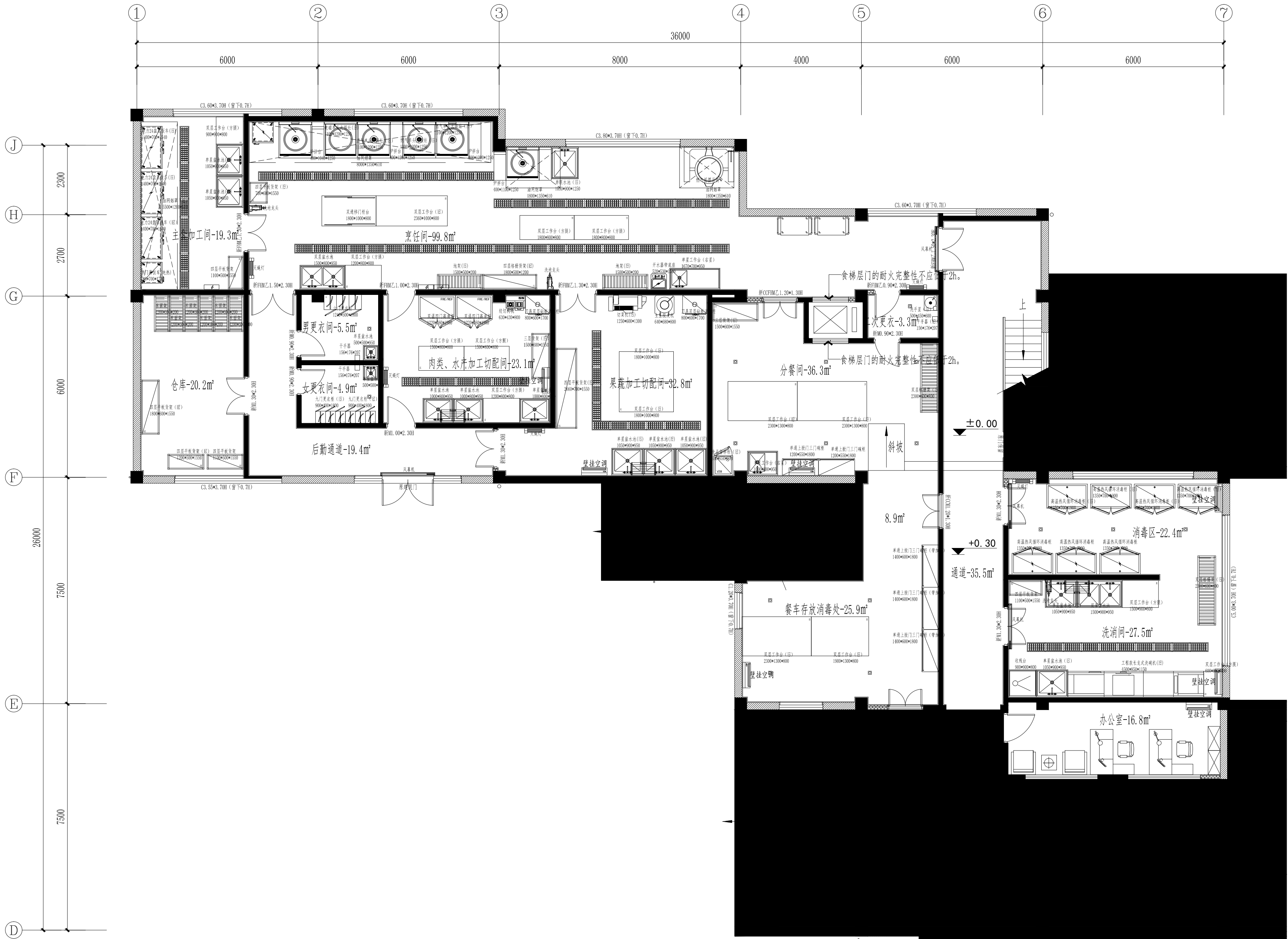
FF 1F FIXTURE/FURNISHING PLAN 一层平面布置图
